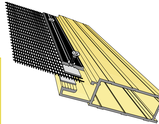
Only Crimsafe drives a screw right through mesh and frame – for unbeatable strength
