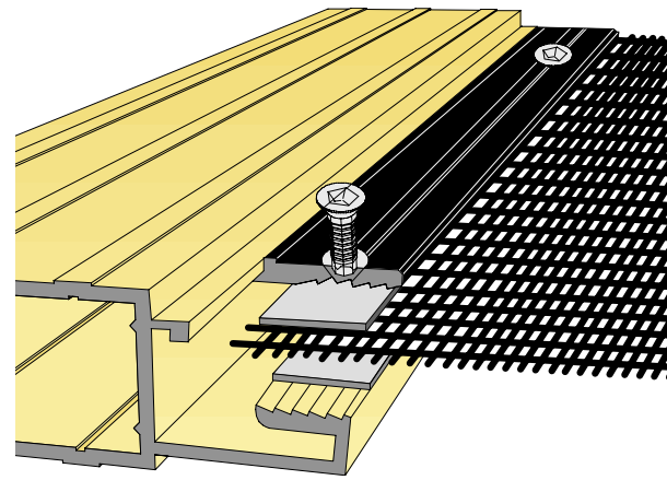
Only Crimsafe drives a screw right through mesh and frame – for unbeatable strength
